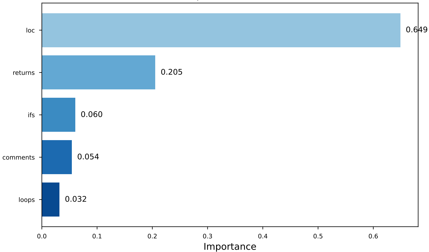
Feature Importance for AI Detection
